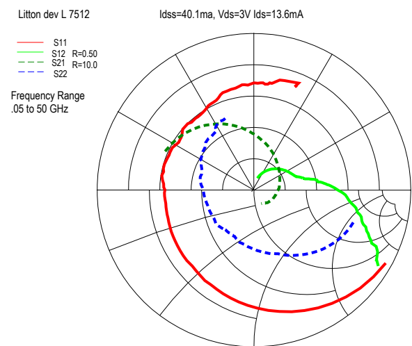
Figure 3. - LP7512 S-Parameters
